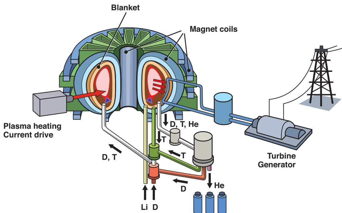
Construction of a tokamak-type fusion power plant (Graphic: MPI for Plasma Physic, Karin Hirl)
